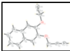
Fig. 1. A view of the title compound, showing the atom-labeling scheme. Displacement ellipsoids are drawn at the 50% probability level and H atoms are shown as small spheres of arbitrary radii.
